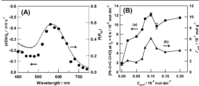
Figure 1. (A) Action spectrum of (dE/dt)_0 (solid circles) and diffuse reflectance UV-vis spectrum of Au/mp-TiO 2 (solid line). (B) Plots of Ph-C=C-CHO concentrations at t_p = 6 h: C_0 = 5 \times 10^{-4} mol dm -3 (a) and adsolubilization amounts of Ph-C=C-CH 2 OH (b) vs C 18 TAC concentration.
