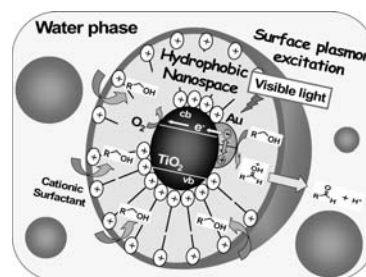
Scheme 1. Self-Assembled Heterosupramolecular Visible Light Photocatalyst
